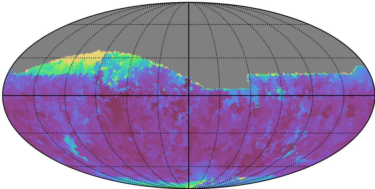
too_5_4v3.4_10yrs Yr 1 i band: Min seeingEff
