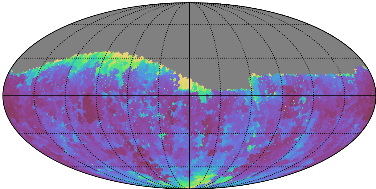
too_5_4v3.4_10yrs Yr 1 g band: Min seeingEff
