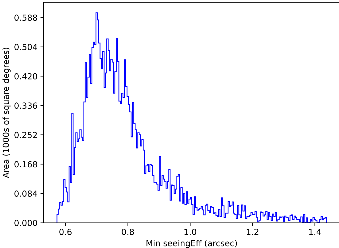
too_5_4v3.4_10yrs Yr 1 g band: Min seeingEff
