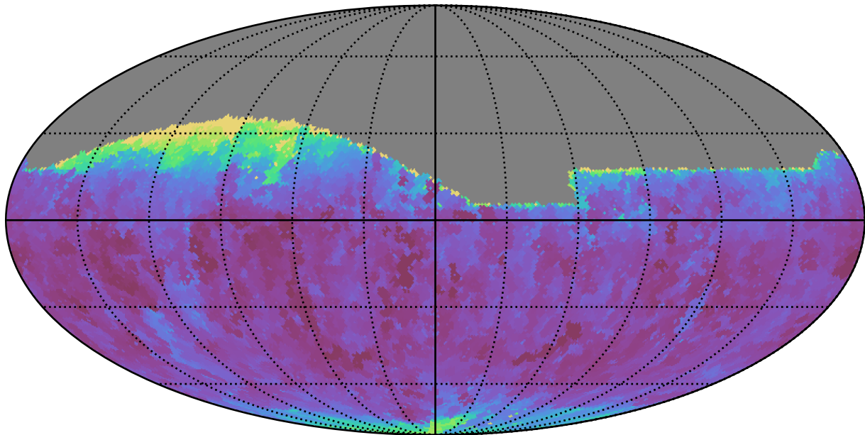
too_5_4v3.4_10yrs Yr 1 all bands: Min seeingEff
