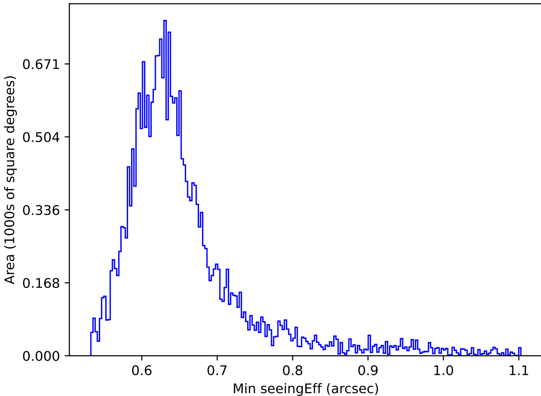
too_5_4v3.4_10yrs Yr 1 all bands: Min seeingEff
