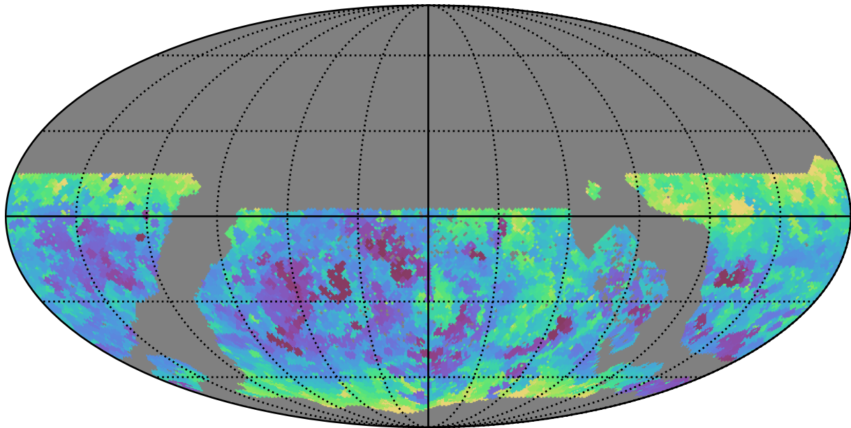
too_5_4v3.4_10yrs WFD z band: Min seeingEff
