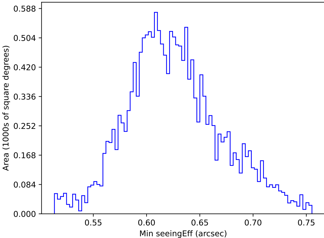
too_5_4v3.4_10yrs WFD y band: Min seeingEff
