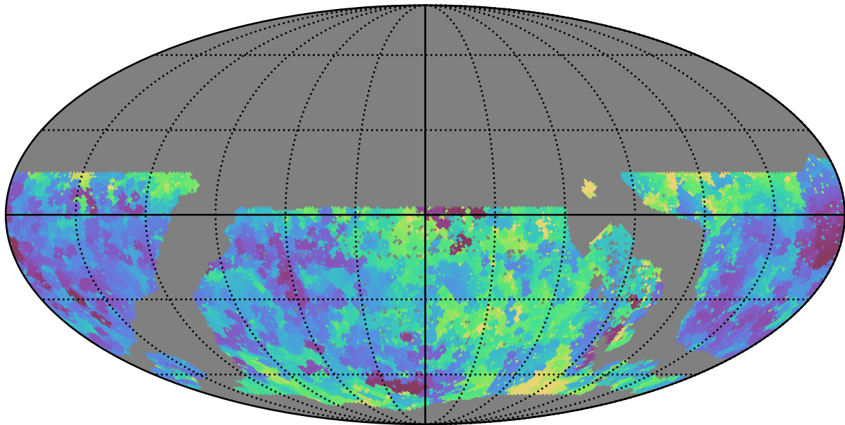
too_5_4v3.4_10yrs WFD u band: Min seeingEff
