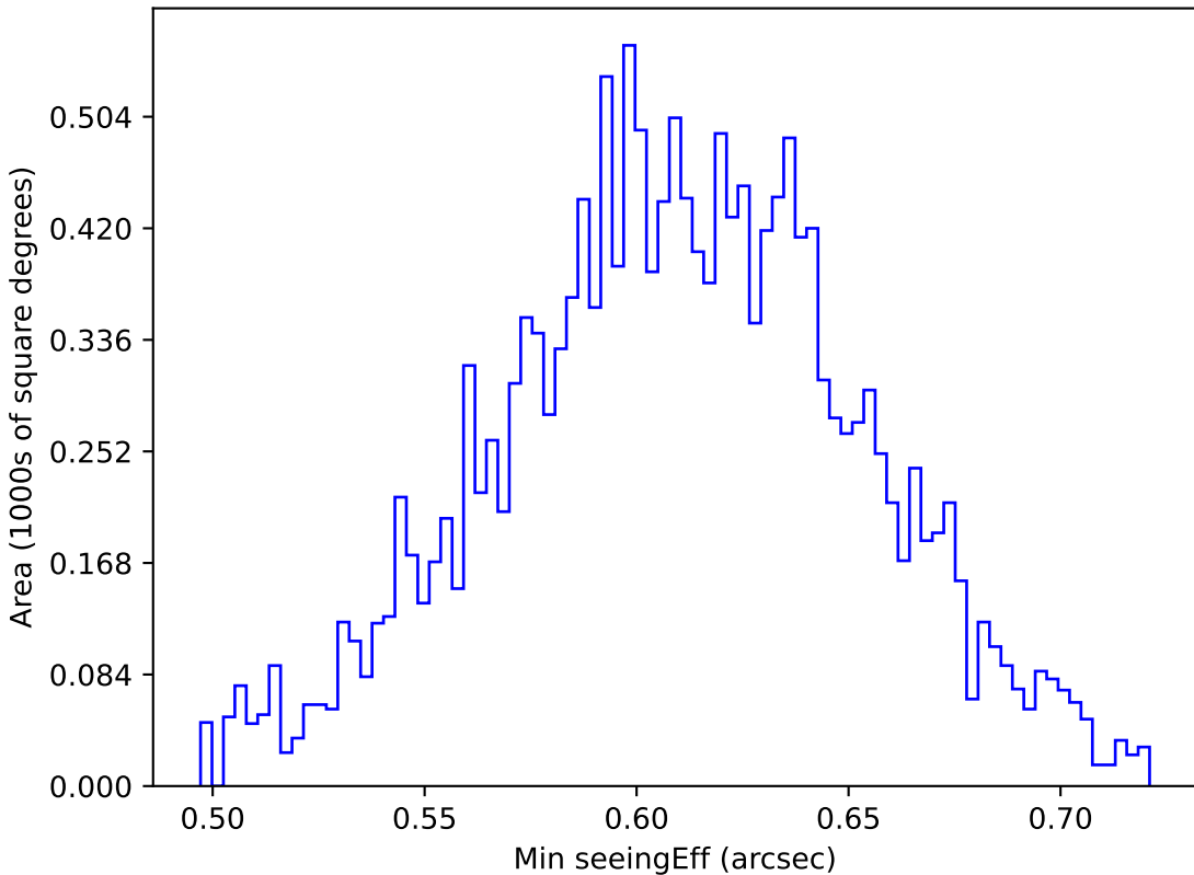
too_5_4v3.4_10yrs WFD r band: Min seeingEff
