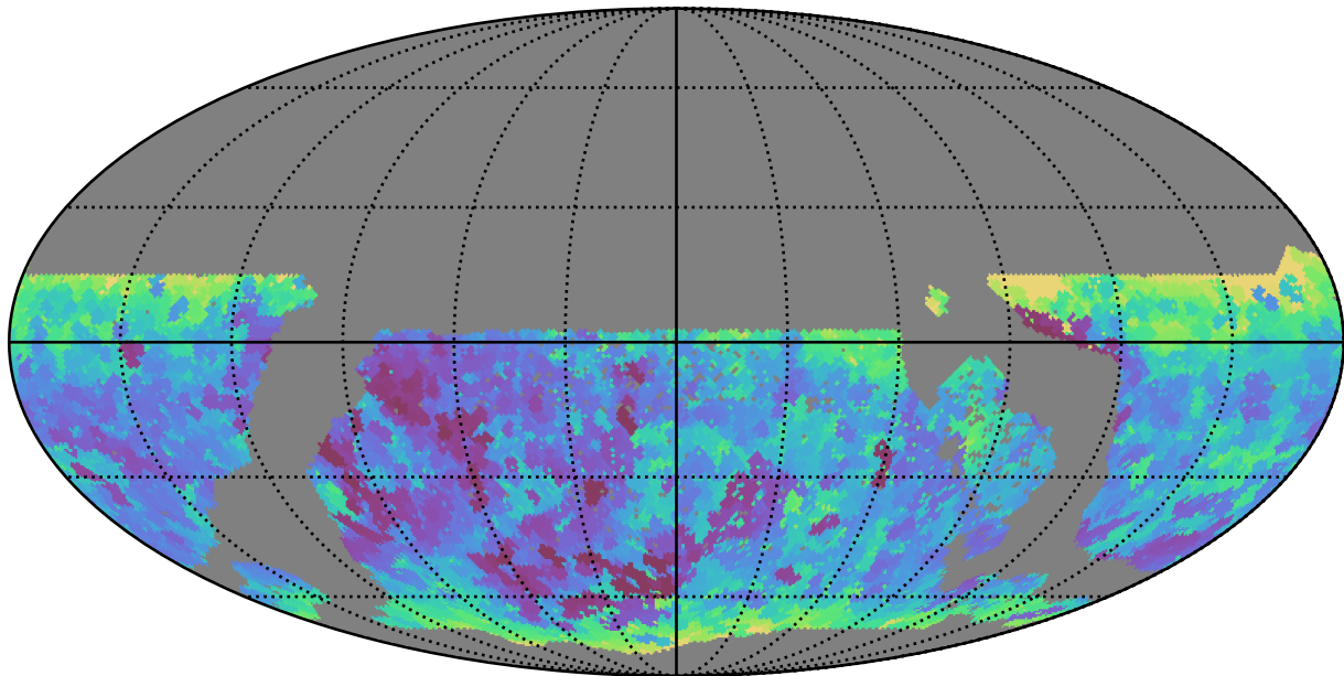
too_5_4v3.4_10yrs WFD i band: Min seeingEff
