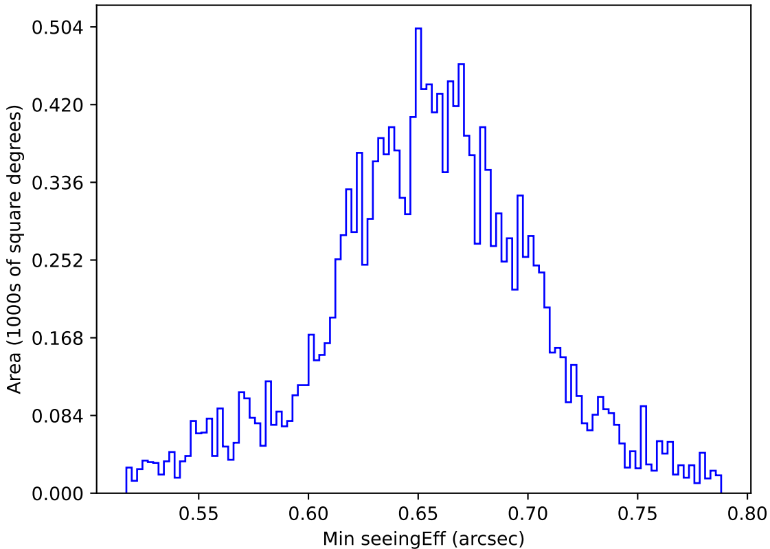
too_5_4v3.4_10yrs WFD g band: Min seeingEff
