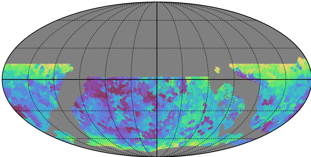
too_5_4v3.4_10yrs WFD all bands: Min seeingEff
