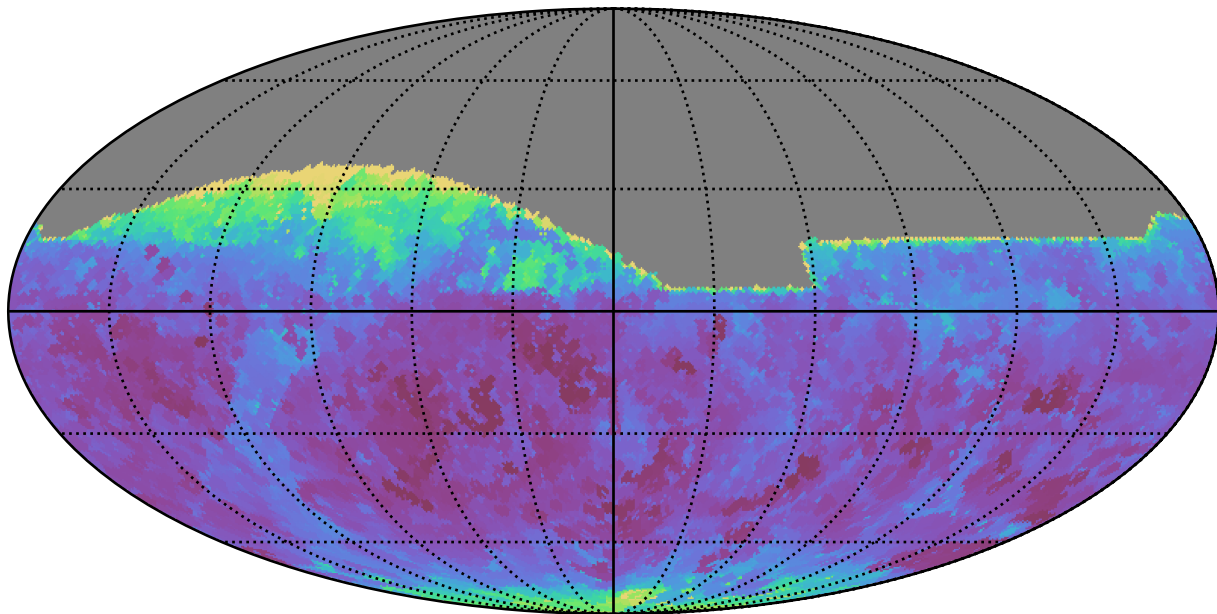
too_5_4v3.4_10yrs All sky z band: Min seeingEff
