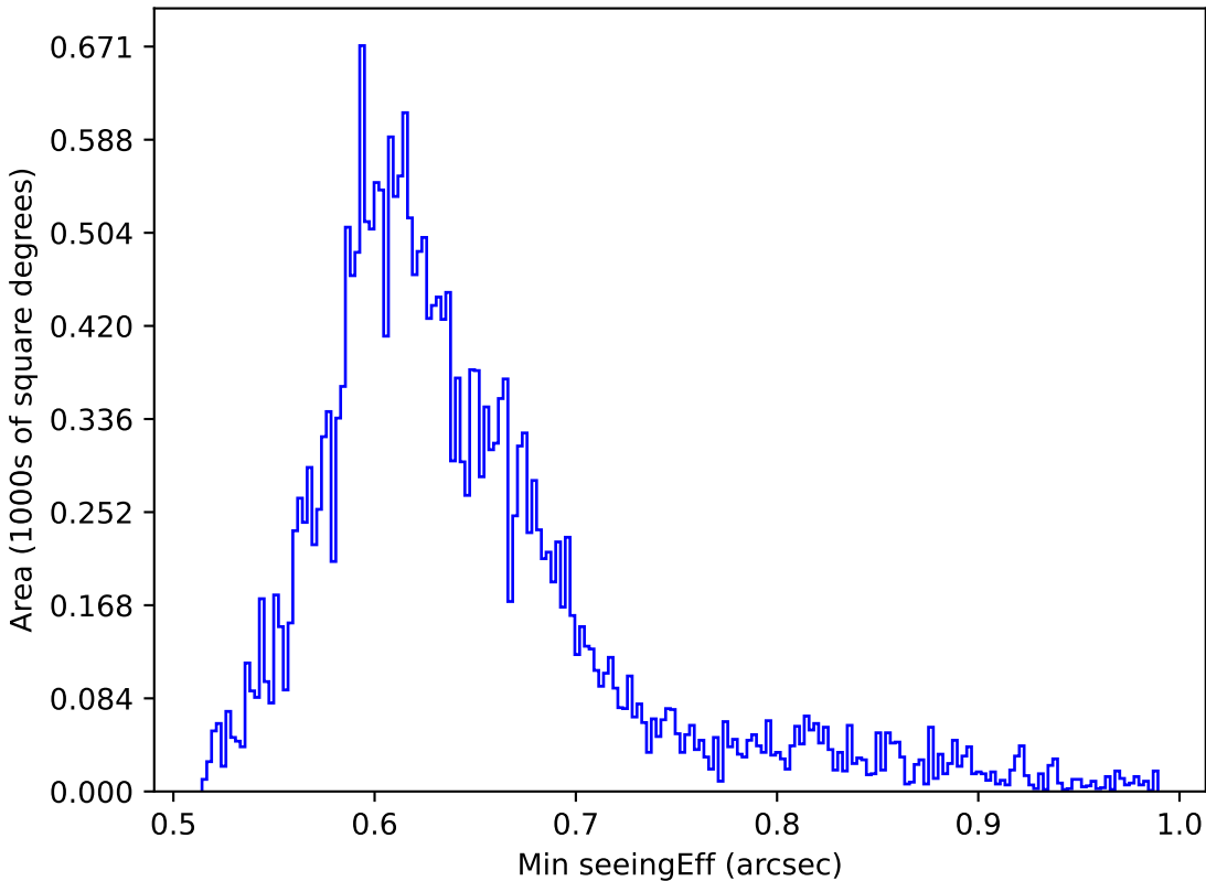
too_5_4v3.4_10yrs All sky z band: Min seeingEff
