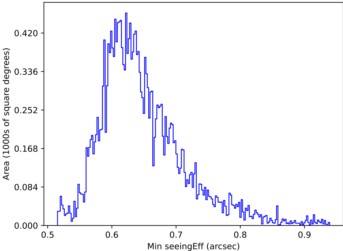
too_5_4v3.4_10yrs All sky y band: Min seeingEff
