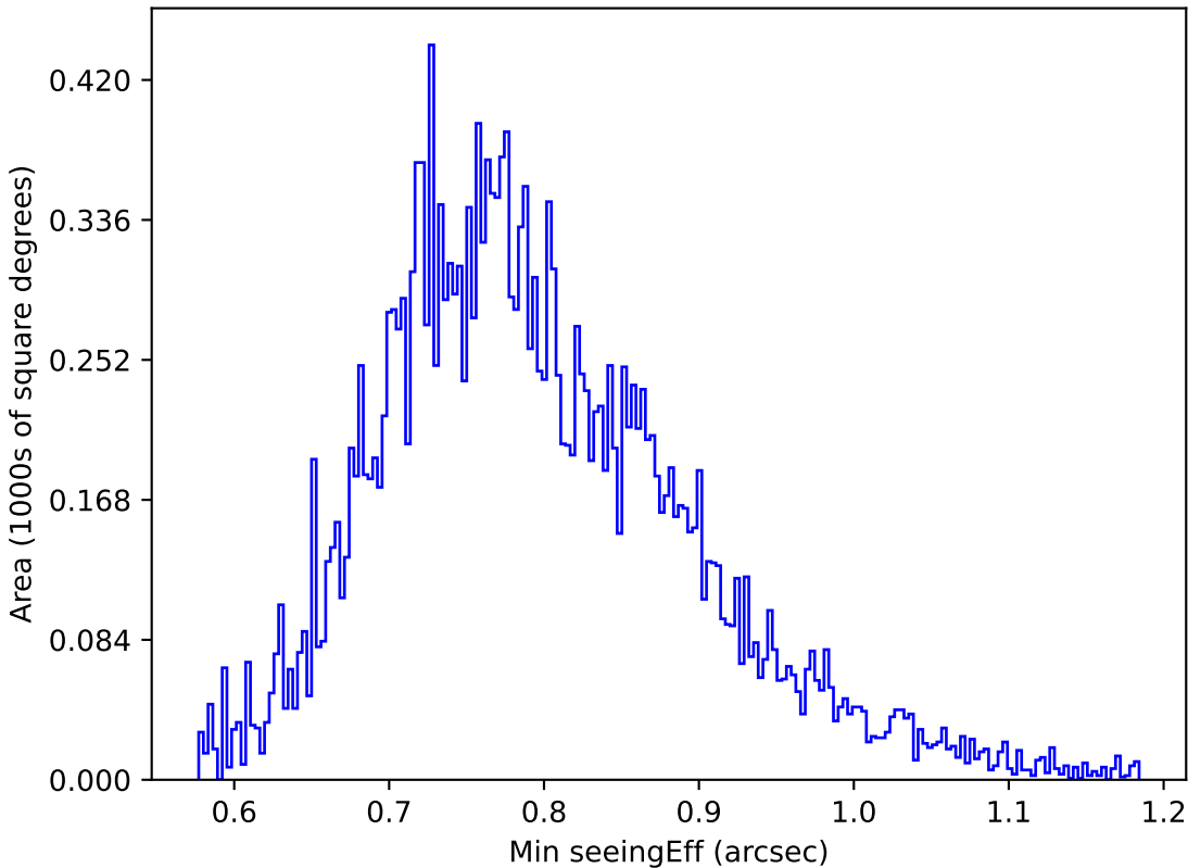
too_5_4v3.4_10yrs All sky u band: Min seeingEff
