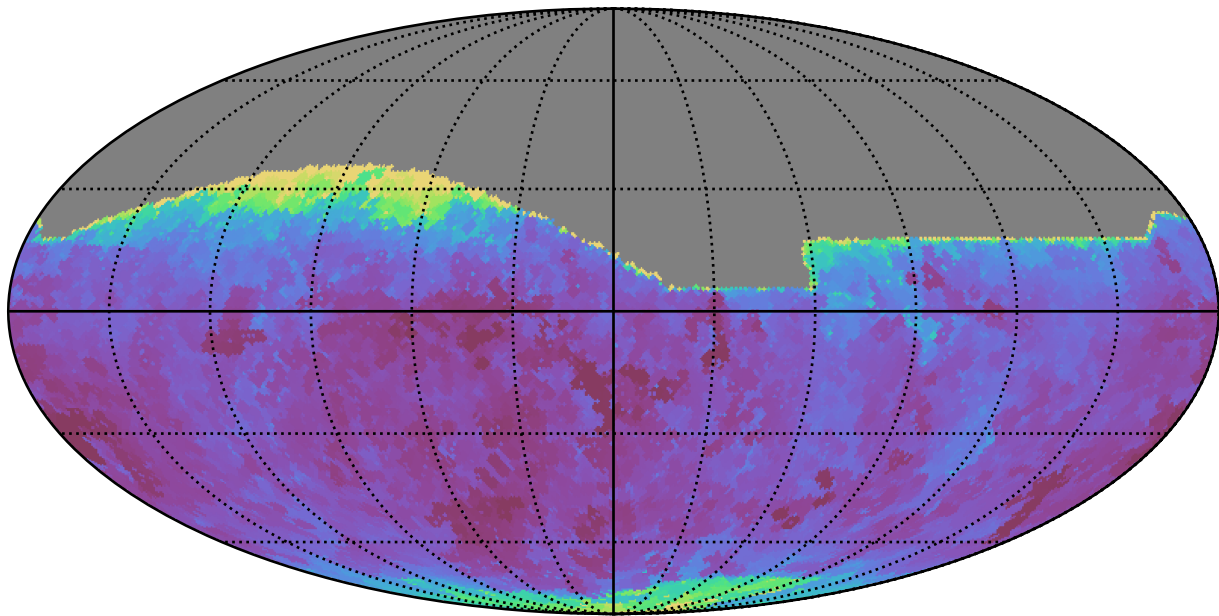
too_5_4v3.4_10yrs All sky r band: Min seeingEff
