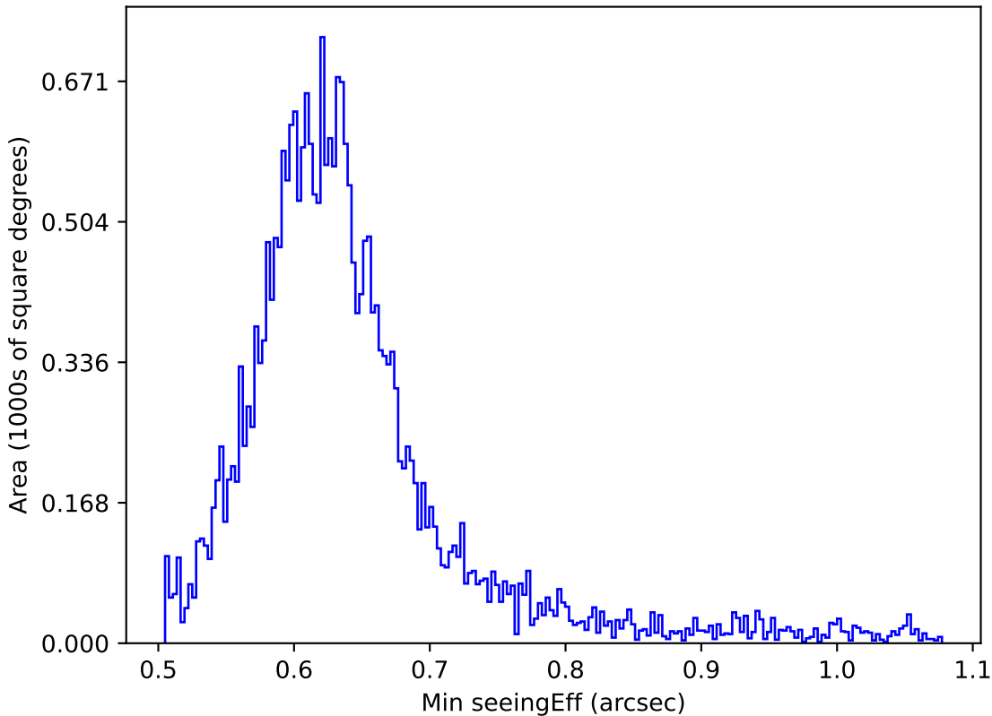
too_5_4v3.4_10yrs All sky r band: Min seeingEff
