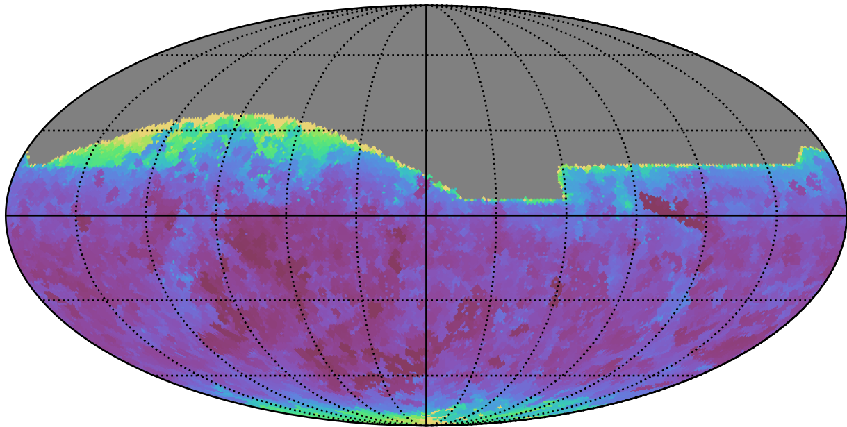
too_5_4v3.4_10yrs All sky i band: Min seeingEff
