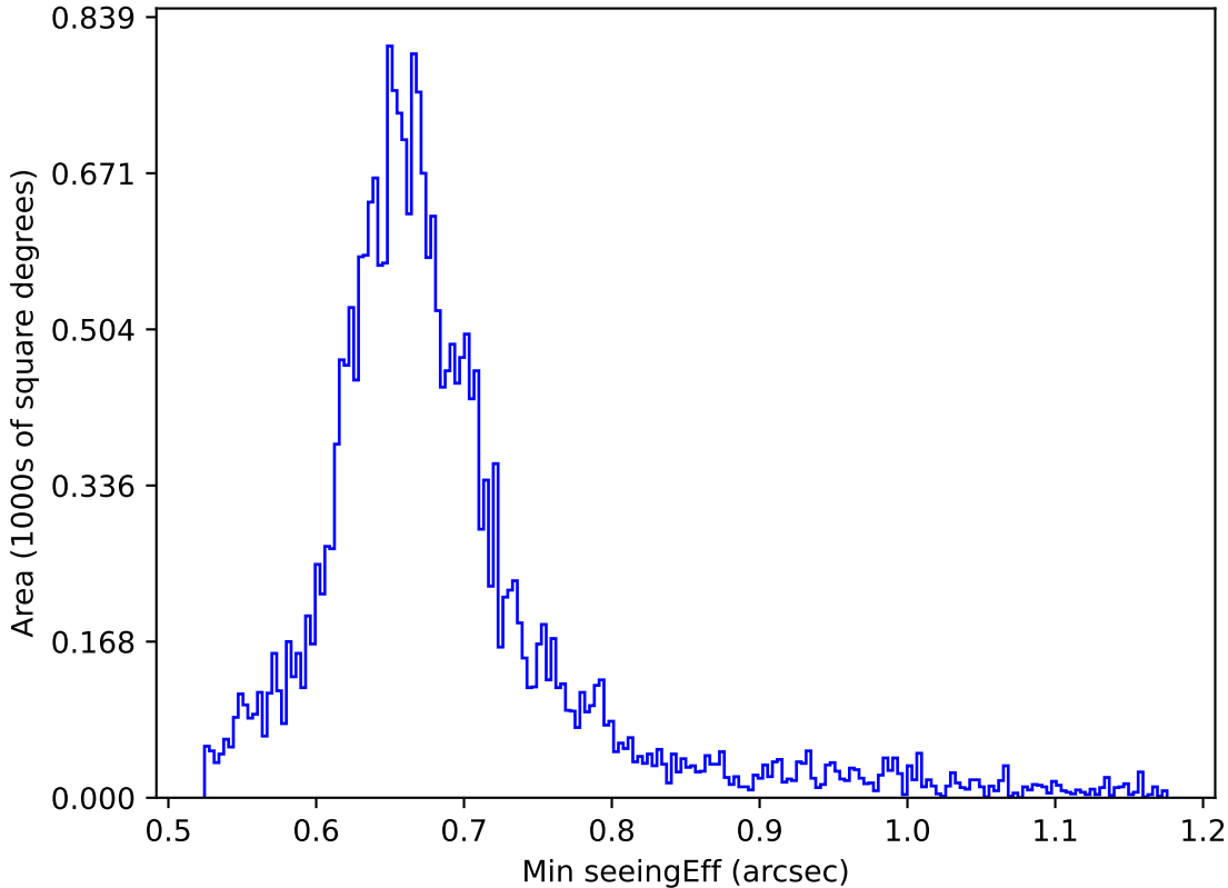
too_5_4v3.4_10yrs All sky g band: Min seeingEff
