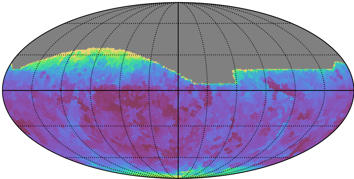
too_5_4v3.4_10yrs All sky all bands: Min seeingEff
