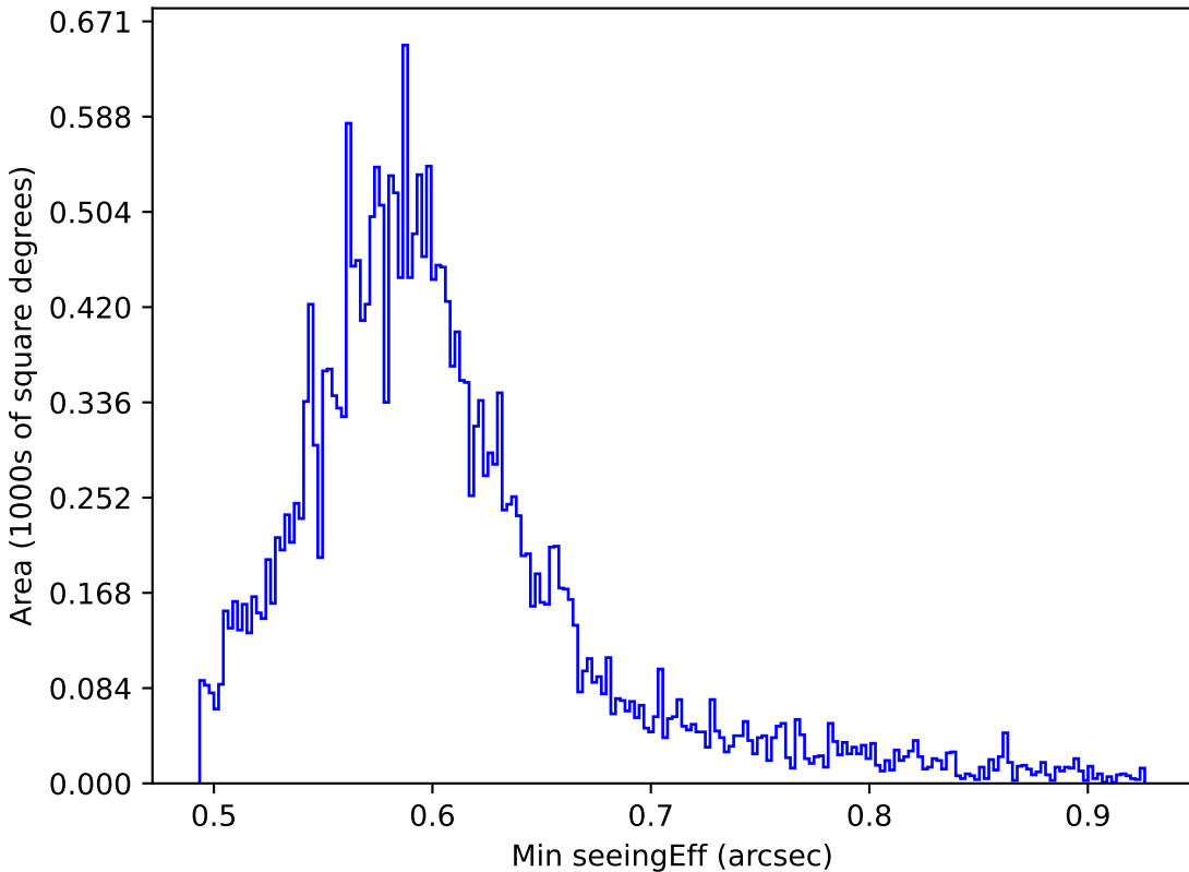
too_5_4v3.4_10yrs All sky all bands: Min seeingEff
