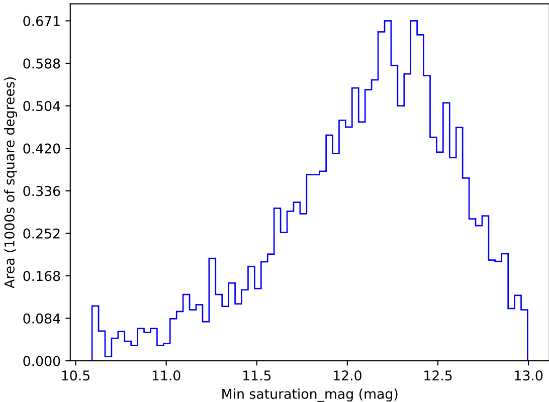
too_5_4v3.4_10yrs WFD z band: Min saturation_mag
