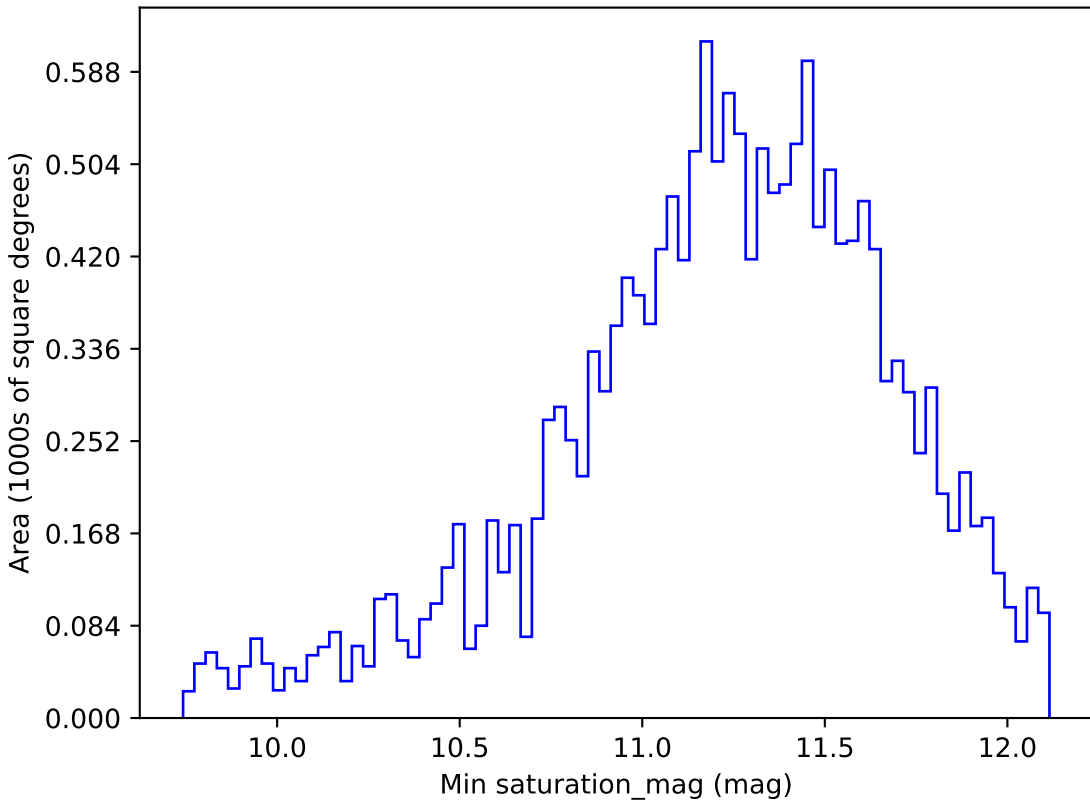
too_5_4v3.4_10yrs WFD y band: Min saturation_mag
