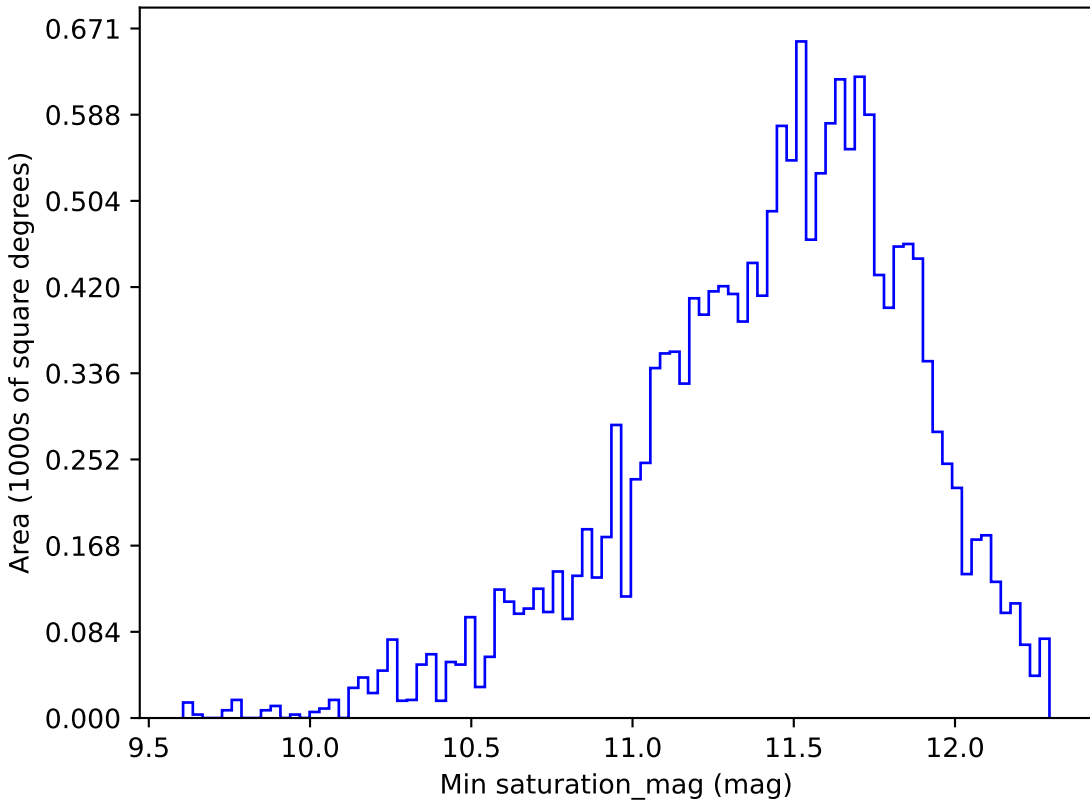
too_5_4v3.4_10yrs WFD u band: Min saturation_mag
