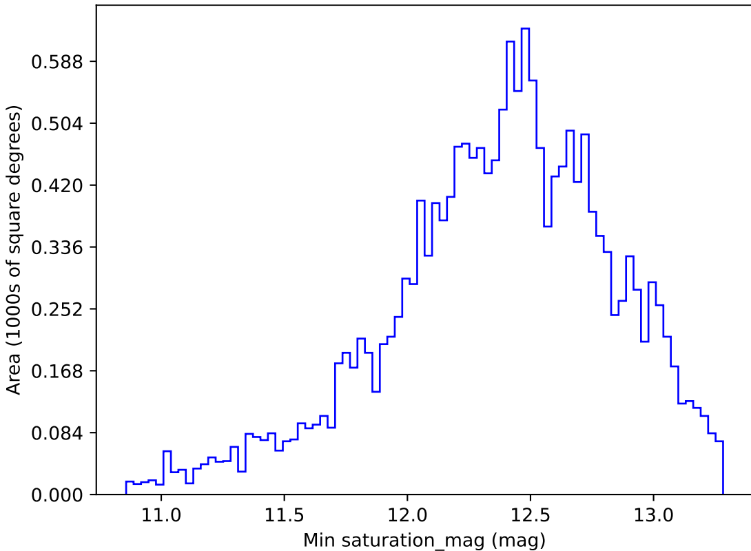
too_5_4v3.4_10yrs WFD i band: Min saturation_mag
