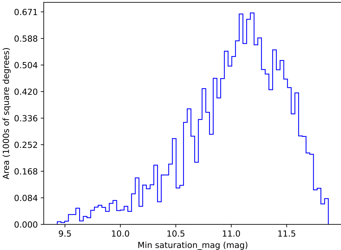
too_5_4v3.4_10yrs WFD all bands: Min saturation_mag
