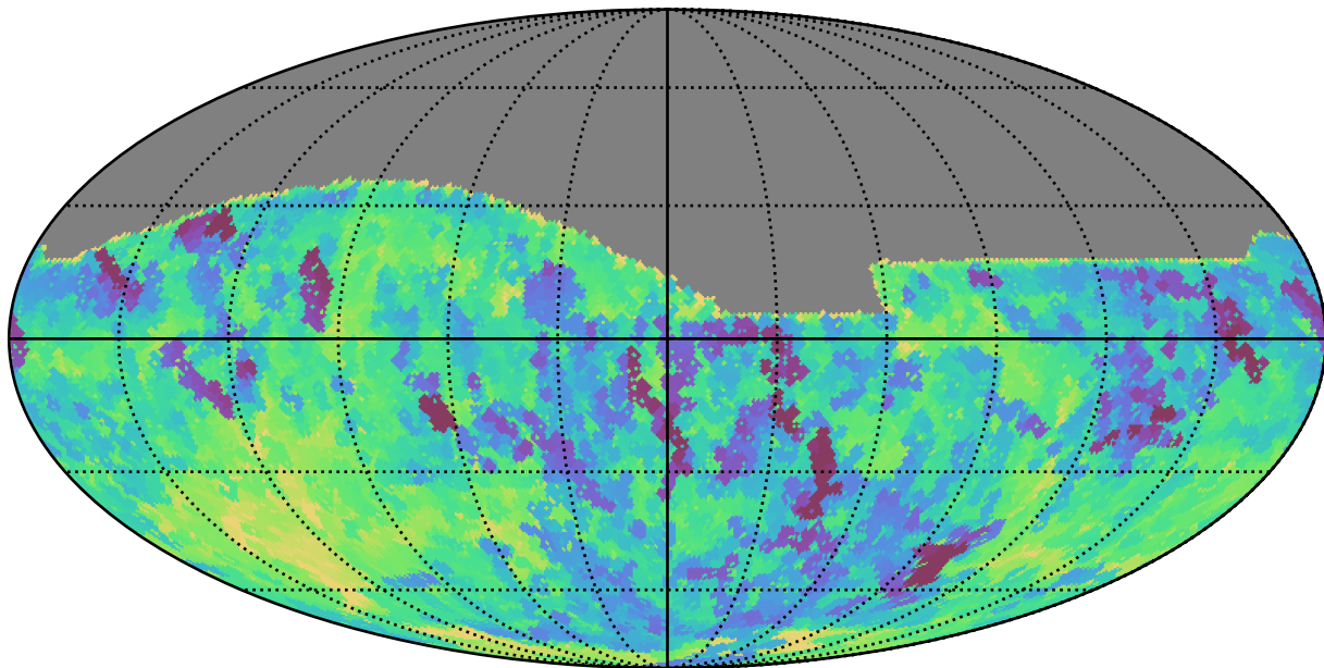
too_5_4v3.4_10yrs All sky z band: Min saturation_mag
