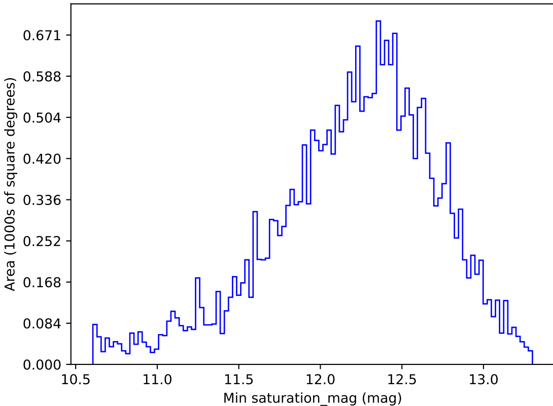
too_5_4v3.4_10yrs All sky z band: Min saturation_mag
