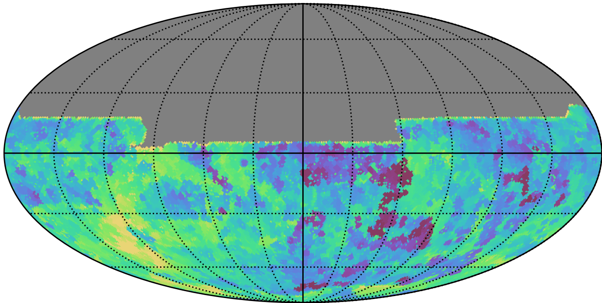
too_5_4v3.4_10yrs All sky y band: Min saturation_mag
