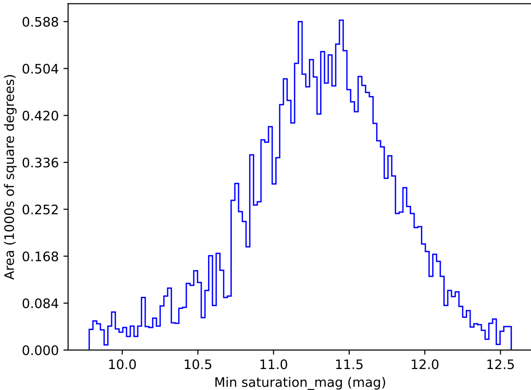
too_5_4v3.4_10yrs All sky y band: Min saturation_mag
