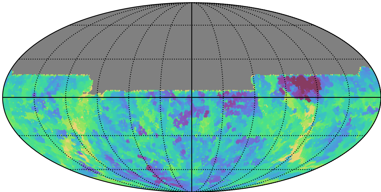
too_5_4v3.4_10yrs All sky u band: Min saturation_mag
