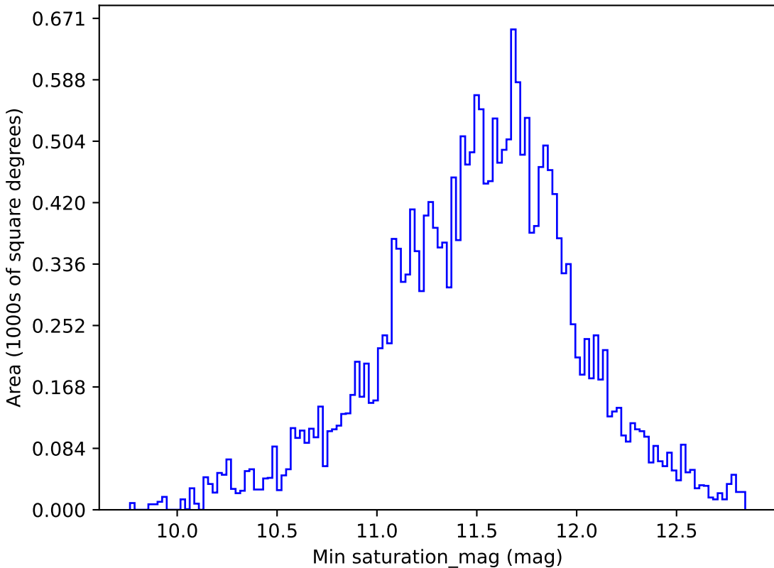
too_5_4v3.4_10yrs All sky u band: Min saturation_mag
