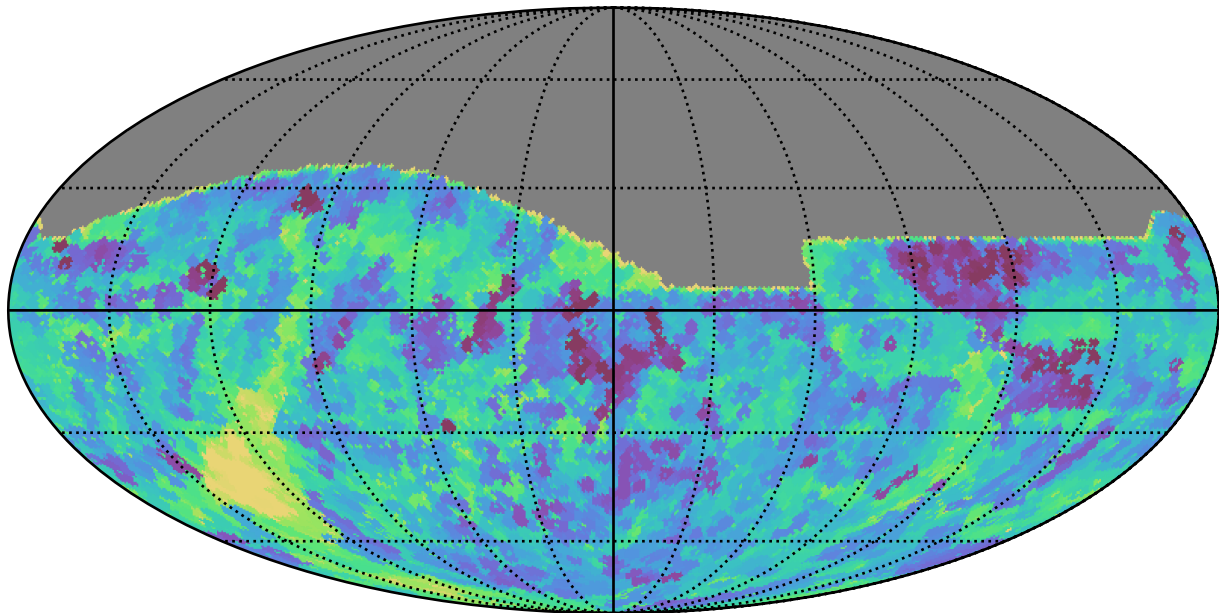
too_5_4v3.4_10yrs All sky r band: Min saturation_mag
