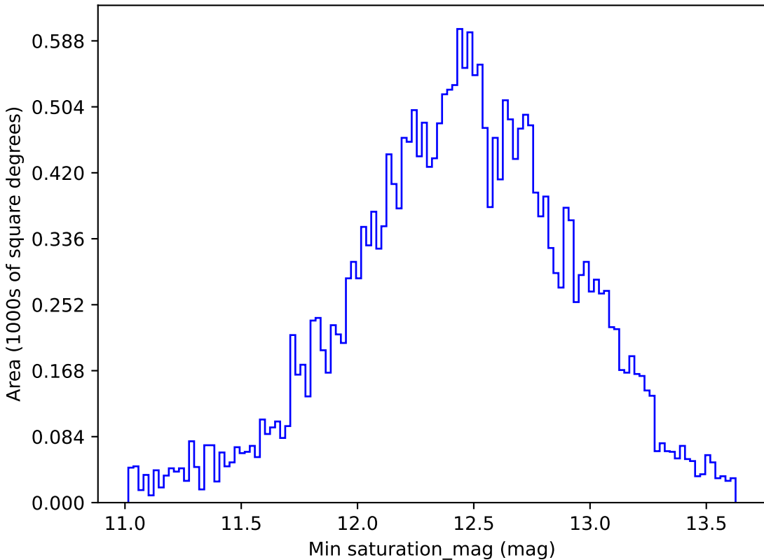
too_5_4v3.4_10yrs All sky i band: Min saturation_mag
