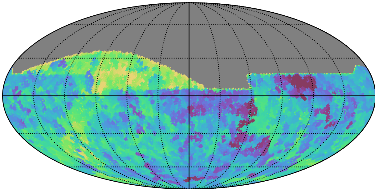
too_5_4v3.4_10yrs All sky all bands: Min saturation_mag
