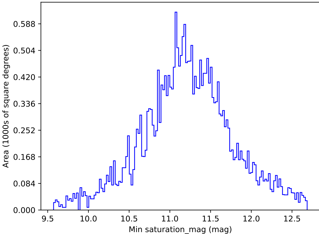
too_5_4v3.4_10yrs All sky all bands: Min saturation_mag
