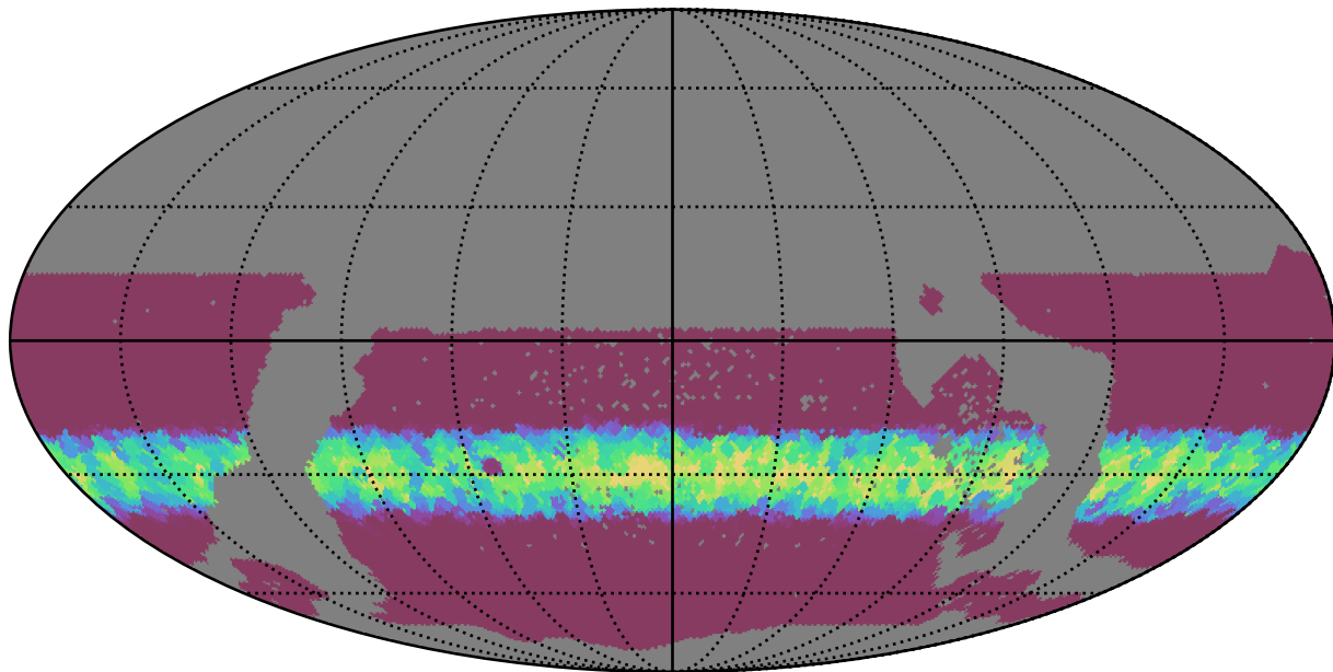
too_5_4v3.4_10yrs WFD r band: Min normairmass
