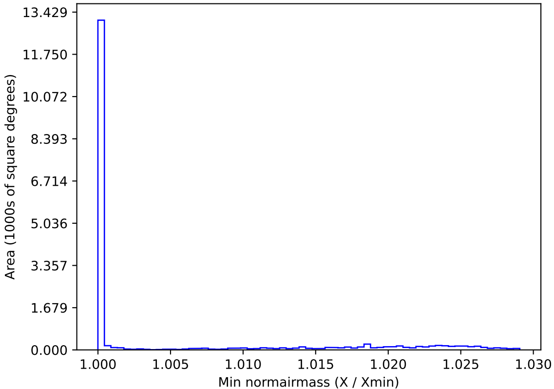
too_5_4v3.4_10yrs WFD all bands: Min normairmass
