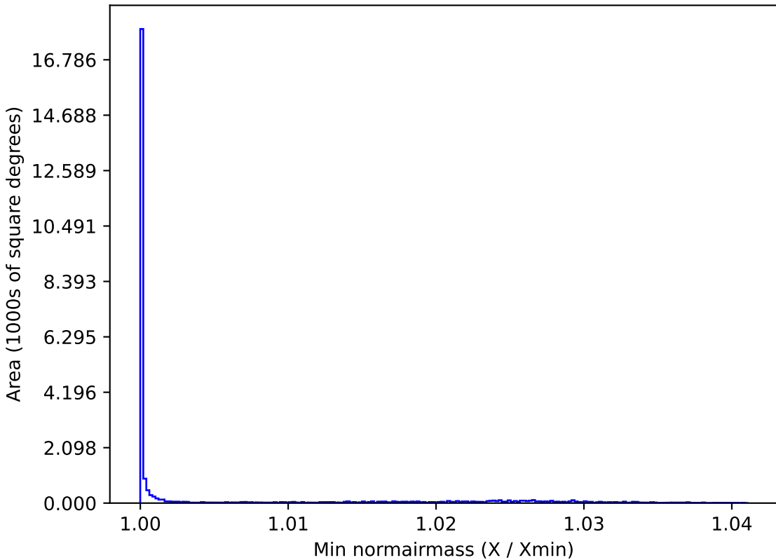
too_5_4v3.4_10yrs All sky z band: Min normairmass
