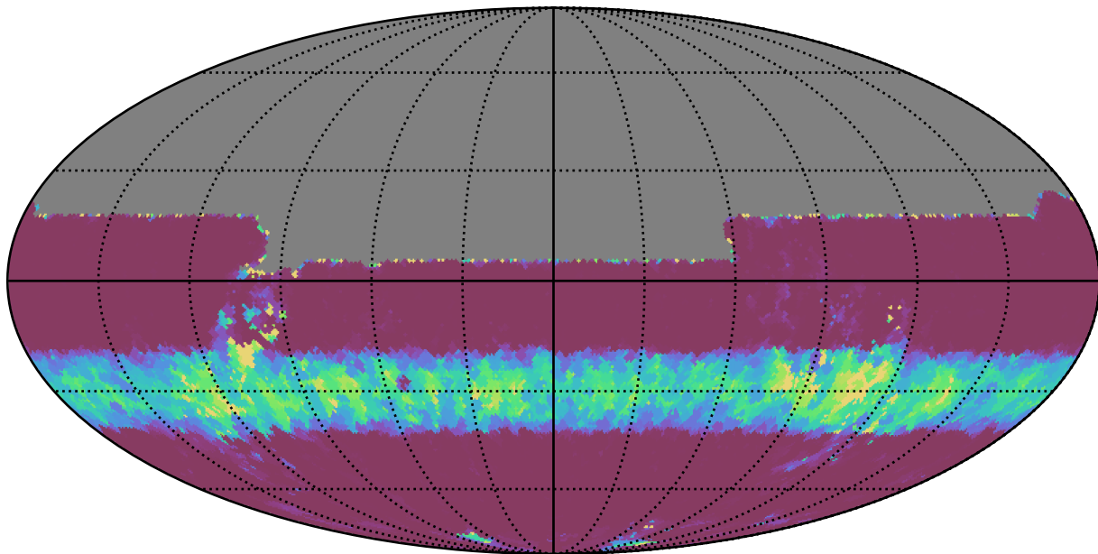
too_5_4v3.4_10yrs All sky u band: Min normairmass
