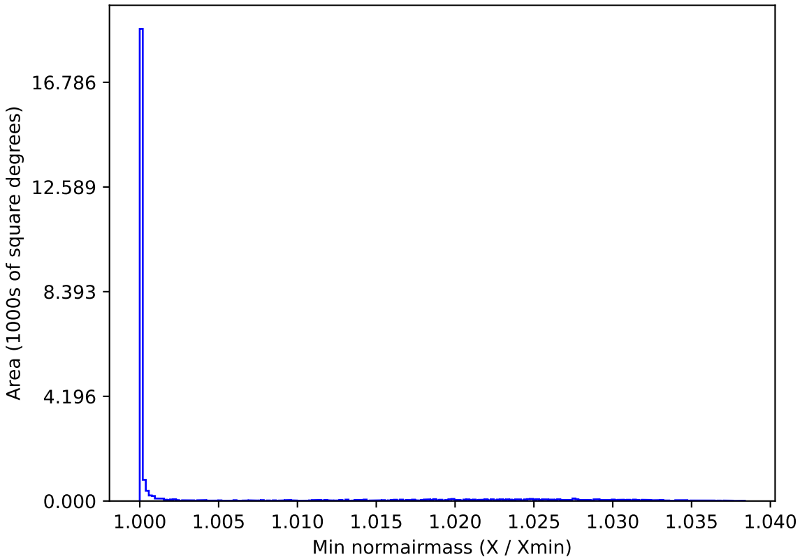
too_5_4v3.4_10yrs All sky r band: Min normairmass
