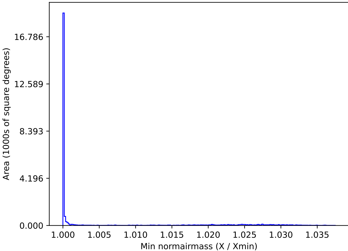
too_5_4v3.4_10yrs All sky i band: Min normairmass
