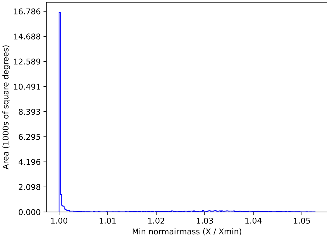
too_5_4v3.4_10yrs All sky g band: Min normairmass
