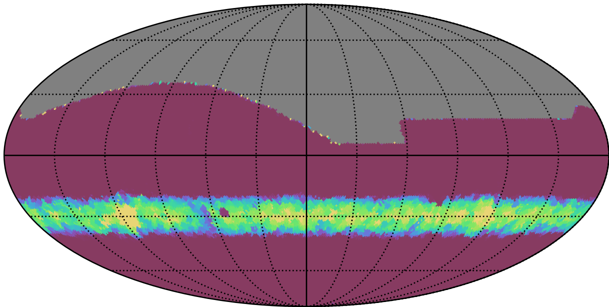
too_5_4v3.4_10yrs All sky all bands: Min normairmass
