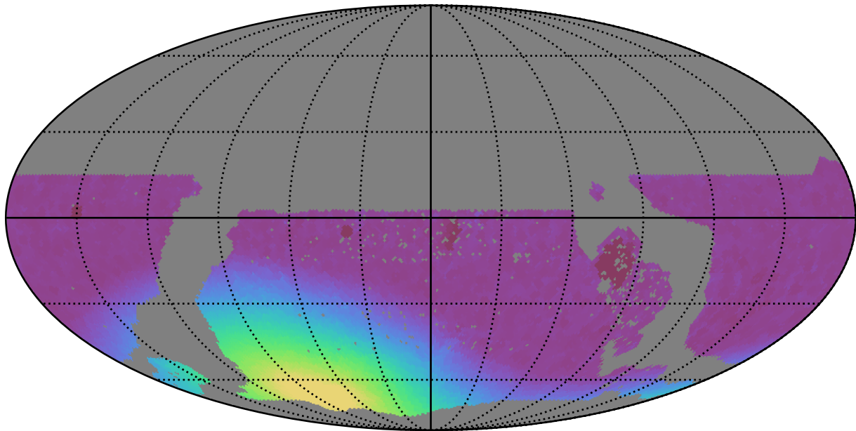
too_5_4v3.4_10yrs WFD z band: Min moonDistance
