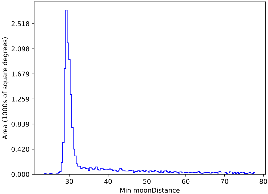
too_5_4v3.4_10yrs WFD z band: Min moonDistance
