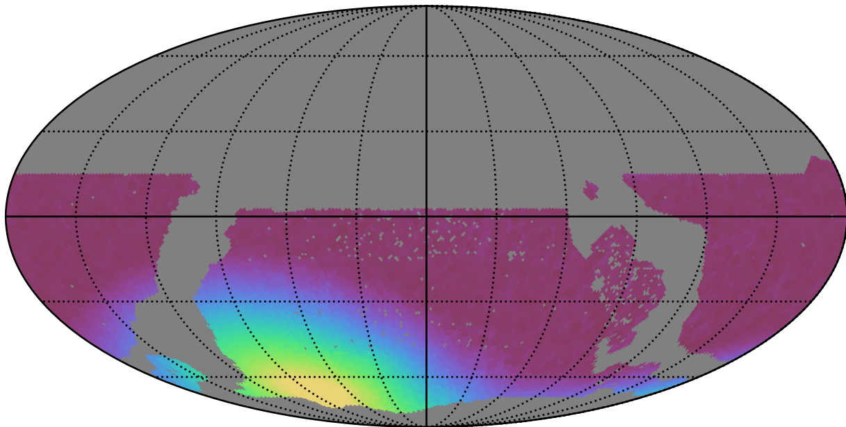
too_5_4v3.4_10yrs WFD y band: Min moonDistance
