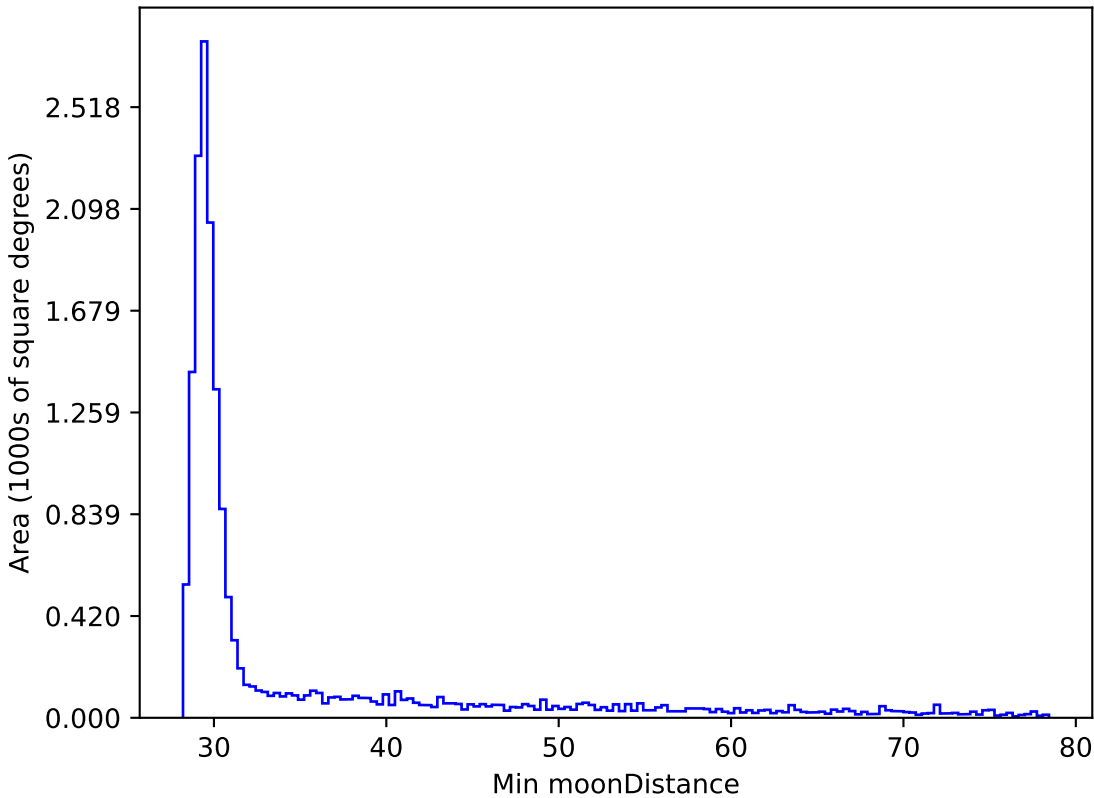
too_5_4v3.4_10yrs WFD y band: Min moonDistance
