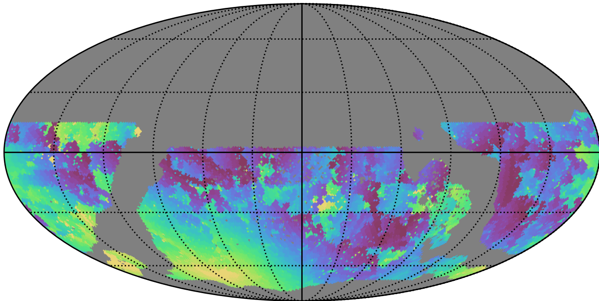
too_5_4v3.4_10yrs WFD u band: Min moonDistance
